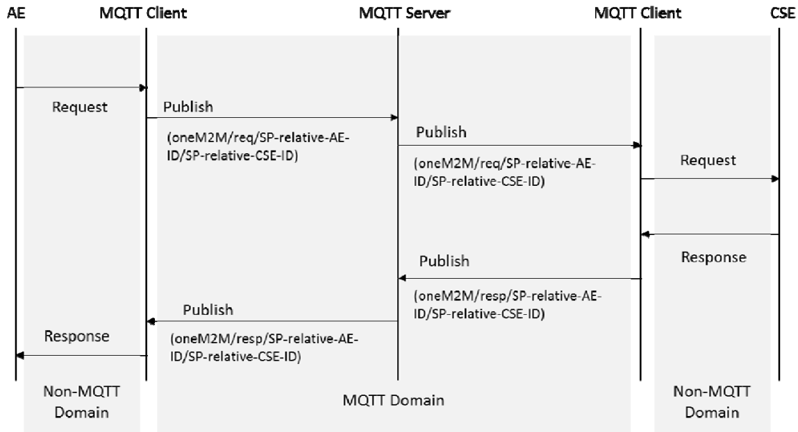
Figure 6.4.5-2: Request/Response message delivery over MQTT
