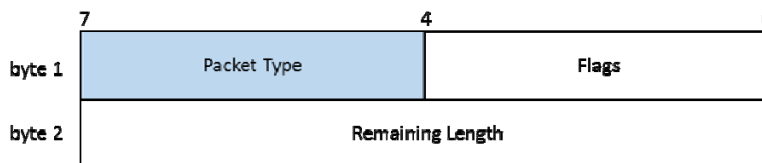
Figure 6.4.1-2: Fixed header structure
