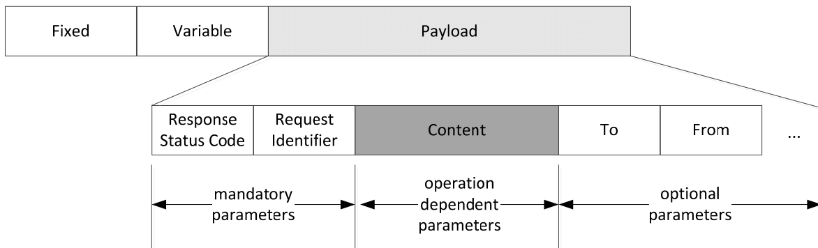
Figure 6.5.2-1: MQTT Response example
