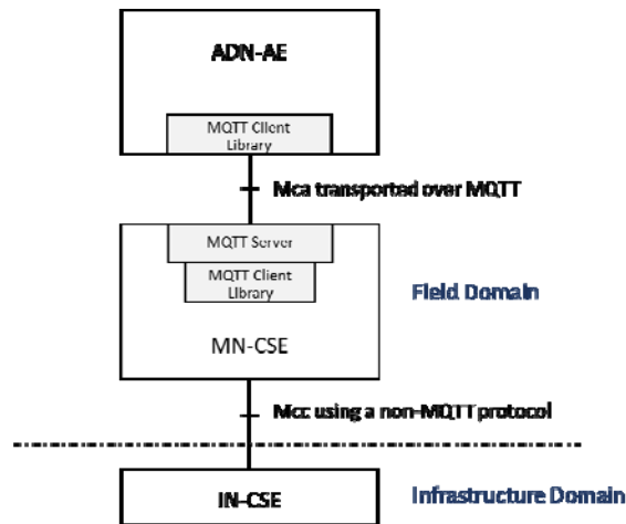
Figure 5.2.3.2-1: Using MQTT between AE and MN-CSE
