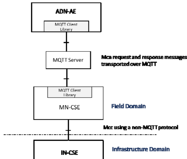
Figure 5.2.3.6-1: Using MQTT between AE and MN-CSE
