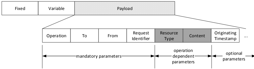
Figure 6.5.1-1: MQTT Request example
