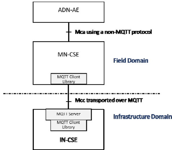
Figure 5.2.3.3-1: Mcc using MQTT between MN and IN
