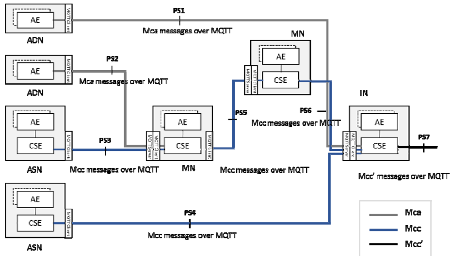
Figure 5.2.2.1-1: MQTT server co-located scenario
