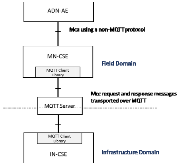
Figure 5.2.3.7-1: Mcc using MQTT between MN and IN
