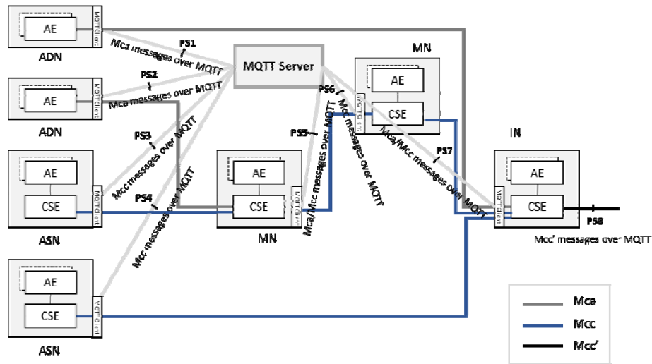
Figure 5.2.2.2-1: MQTT server independently located scenario
