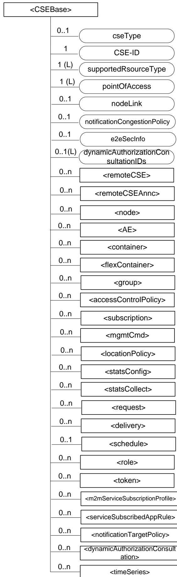
Figure 9.6.3-1: Structure of <CSEBase> resource © oneM2M Partners Type 1 (ARIB, ATIS, CCSA, ETSI, TTA, TSDSI, TTA, TTC) Page 122 of 427
