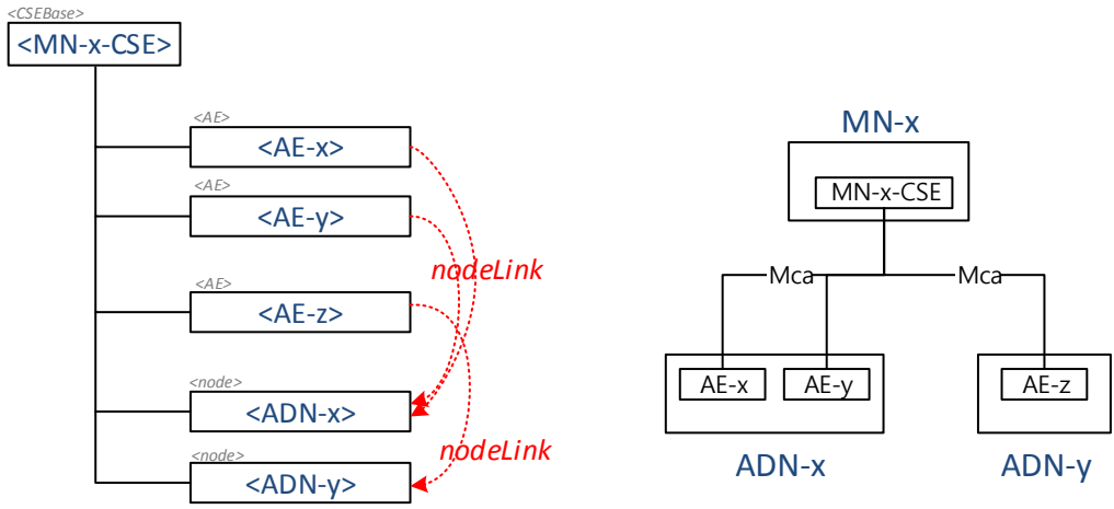
Figure 9.6.18-1: Relationship between MN and ADN
