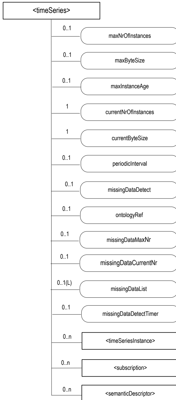
Figure 9.6.36-1: Structure of <timeSeries> resource
