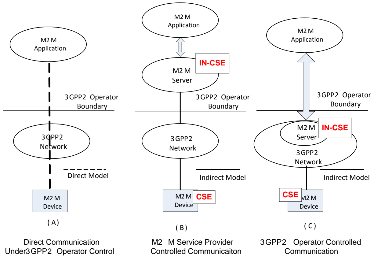
Figure C.2-1: M2M Communication Models
