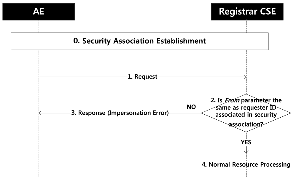
Figure 7.2-1: AE impersonation checking procedure
